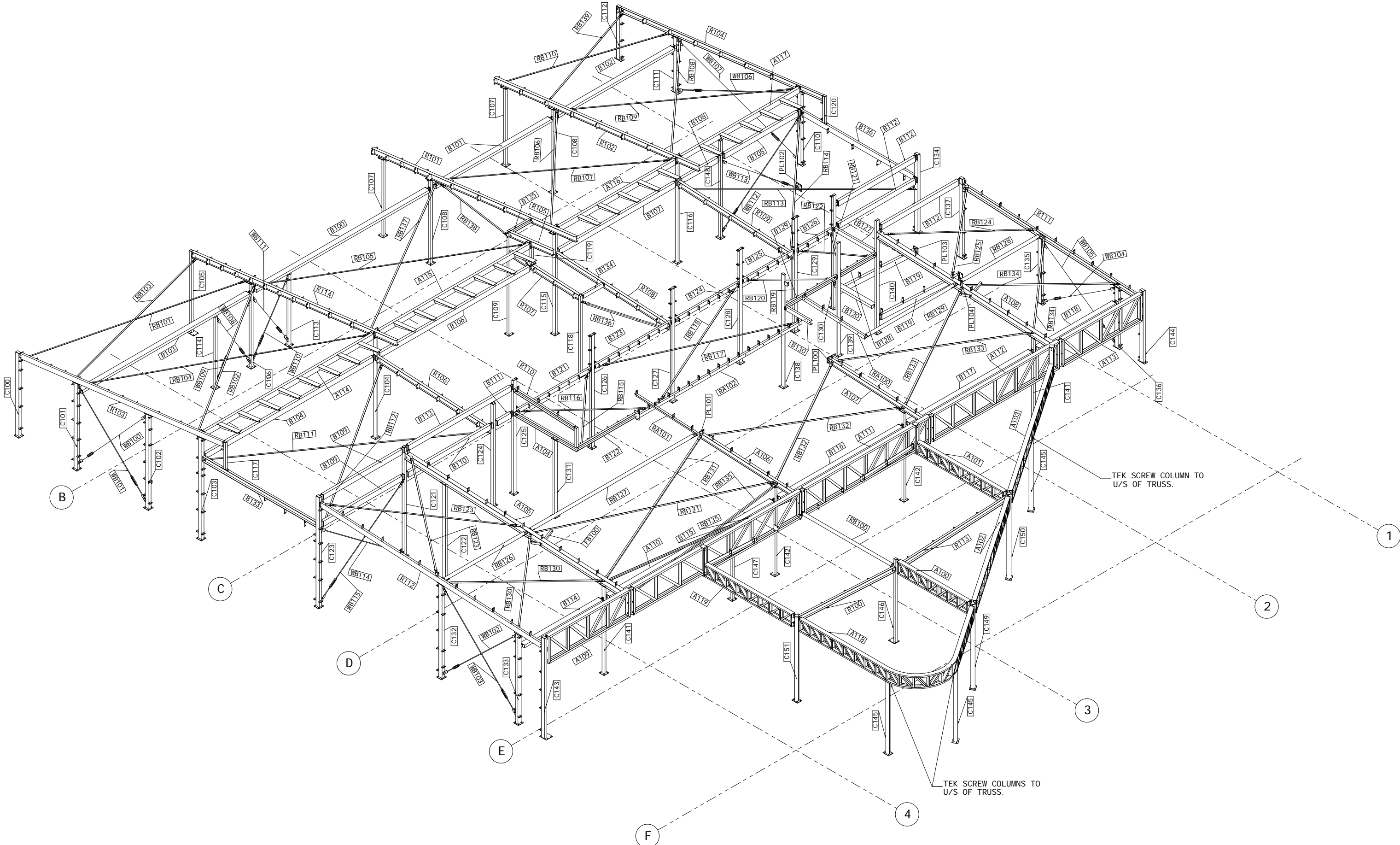
3-D VIEW
